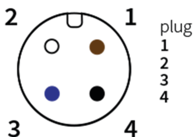
M12 plug 4 pin (standard)
