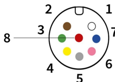
M12 plug 8 pin (extended functions)
